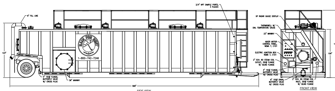
Drawing for 2014-forward model.
